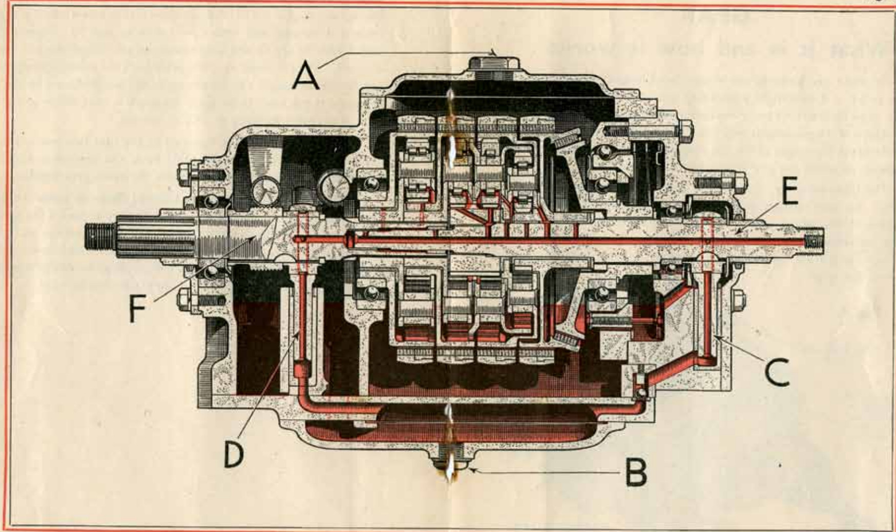
This is a full-length section of a WILSON GEAR BOX showing the oil level and the circulatory system which reaches to all moving parts, (A) is the oil filler cap, (B) the drain plug, (C) the forward oil pump, (D) the rear oil pump, (E) the input shaft, and (F) the output shaft, which transmits the drive to the back axle.
