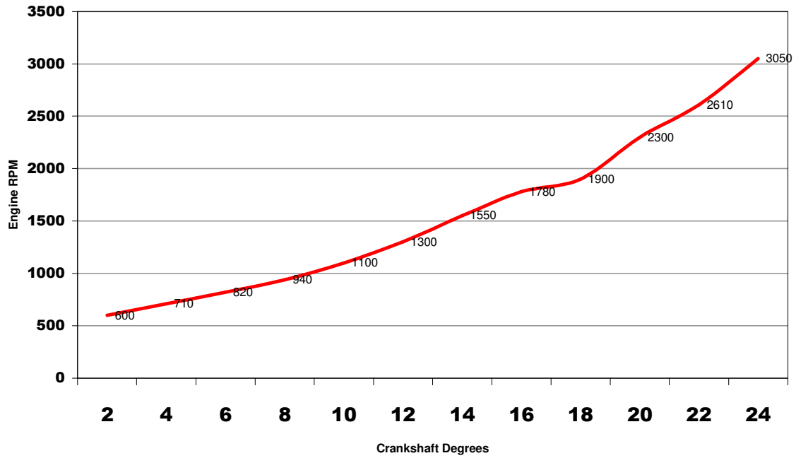
A/B Advance Curve P/N: D177600/D179600/D171600
