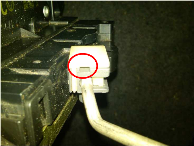
White Plastic Connector Closed, Clamped Around Metal Linkage Red circle marks opening to pry apart with small screwdriver
