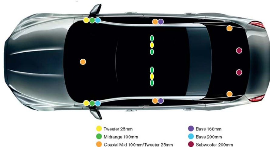
Meridian Reference Audio System – 26 Speakers locations
