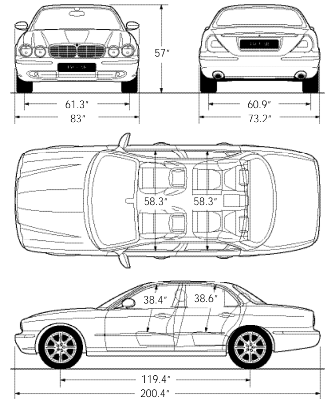
Dimensions shown in inches.
