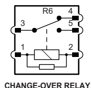
CHANGE-OVER RELAY
