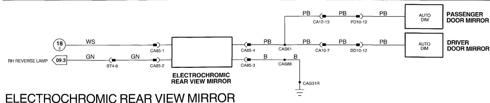
ELECTROCHROMIC REAR VIEW MIRROR
