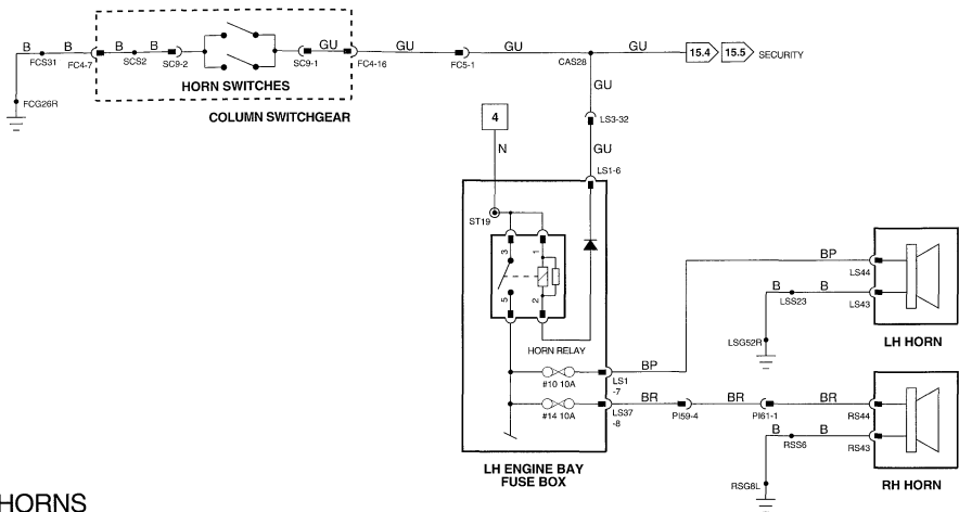
HORNS
