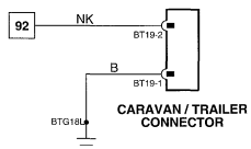
CARAVAN / TRAILER CONNECTOR
