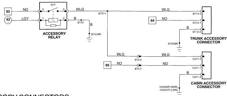
ACCESSORY CONNECTORS
