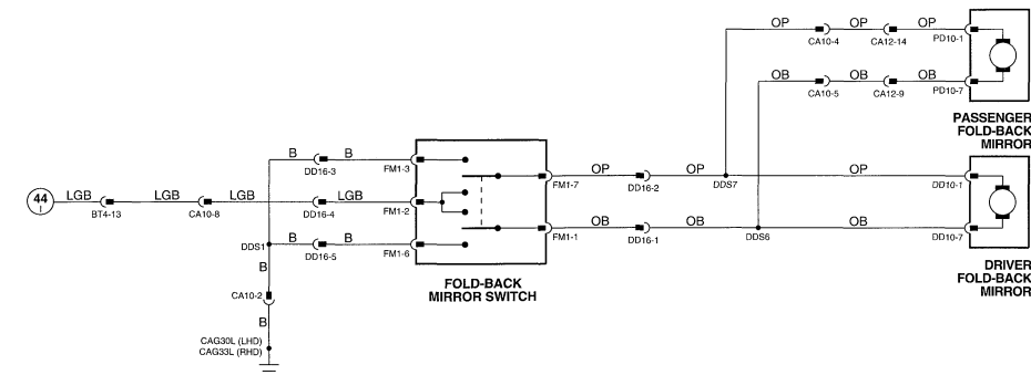
FOLD-BACK MIRRORS
