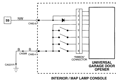
UNIVERSAL GARAGE DOOR OPENER
