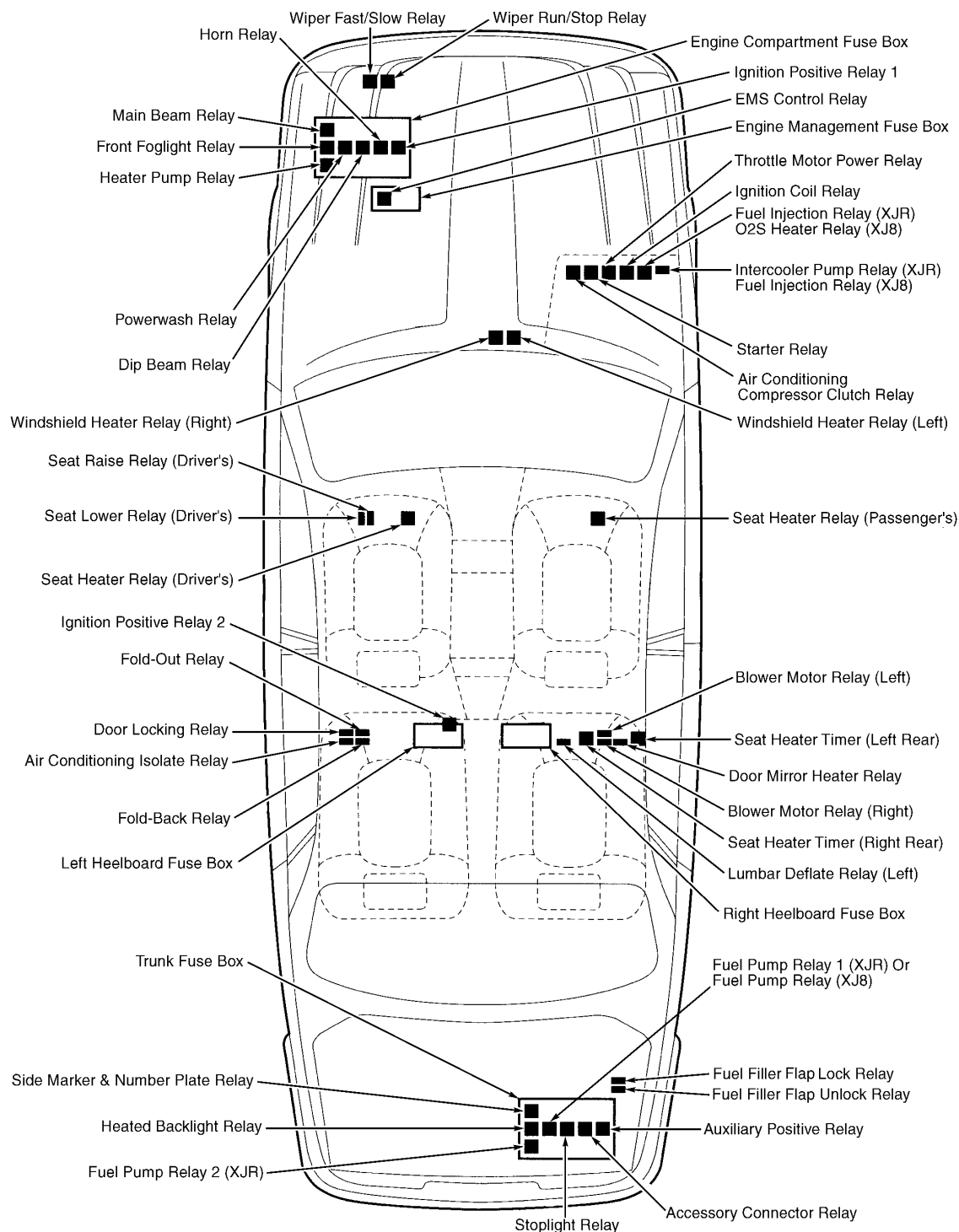
Fig. 1: Vehicle Overview
