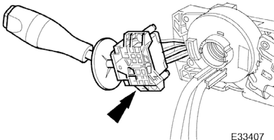
15. Remove flasher/lamp/trip switch assembly from switchgear bracket.
