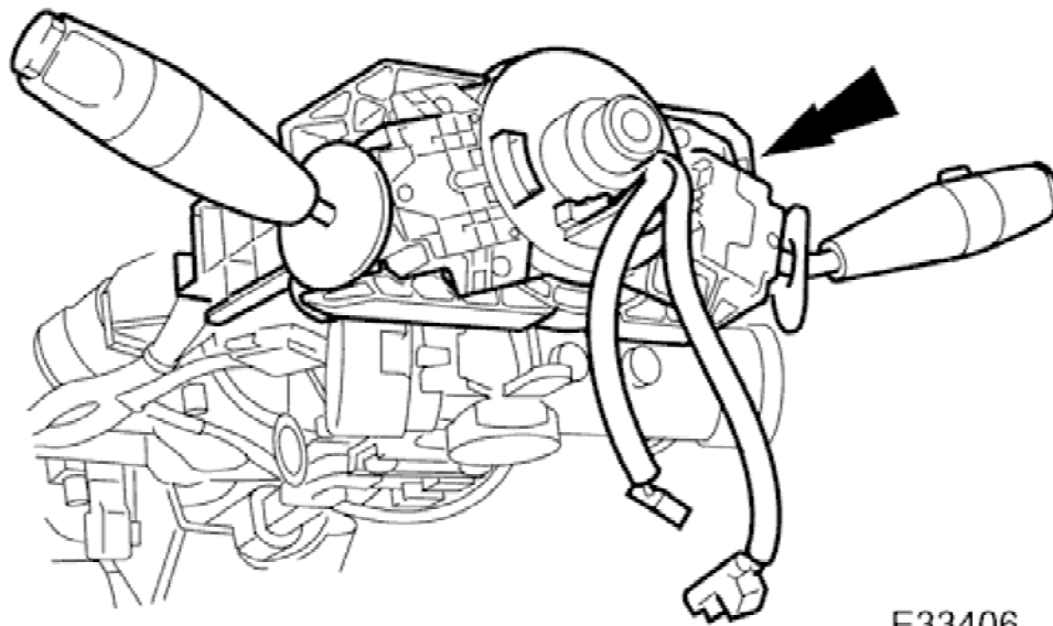
14. Remove steering column switchgear assembly for access.
