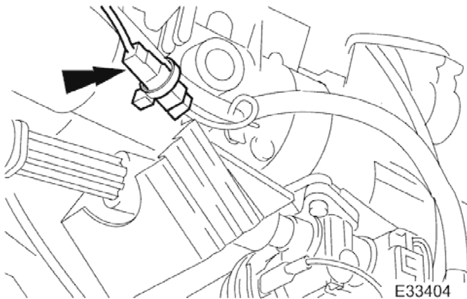
10. Disconnect key interlock solenoid harness multiplug.
