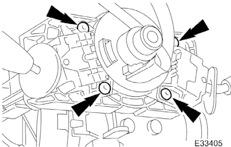
13. Slacken and remove bolts securing switch assemblies/cancellation module to column.
