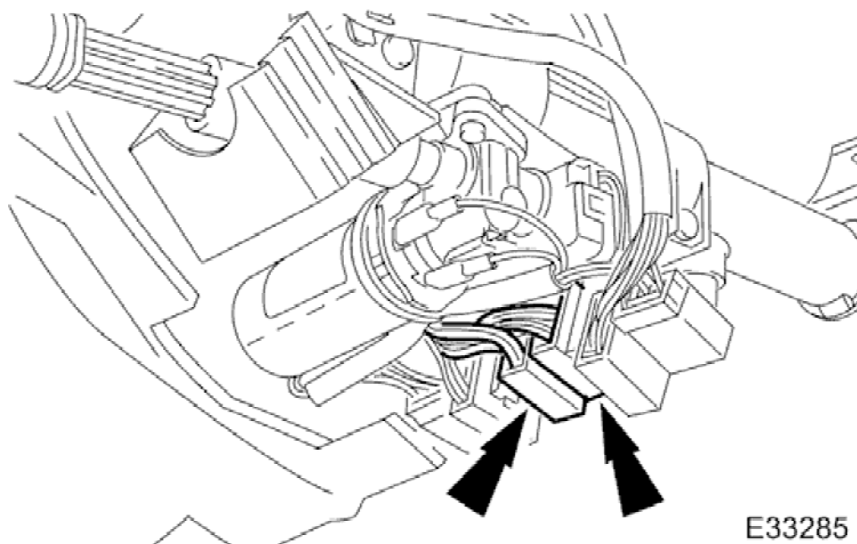
11. Release flasher/lamp/trip switch harness multiplugs from retaining bracket and disconnect multiplugs.
