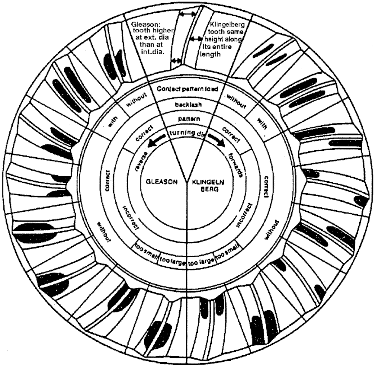
Fig. 22 Ring Gear Pinion Tooth Contact Correction Chart
