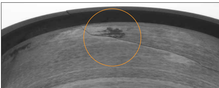
Fig. 52. This ball bearing inner ring fracture results from installation on top of a metal contaminant or raised metal nick.
