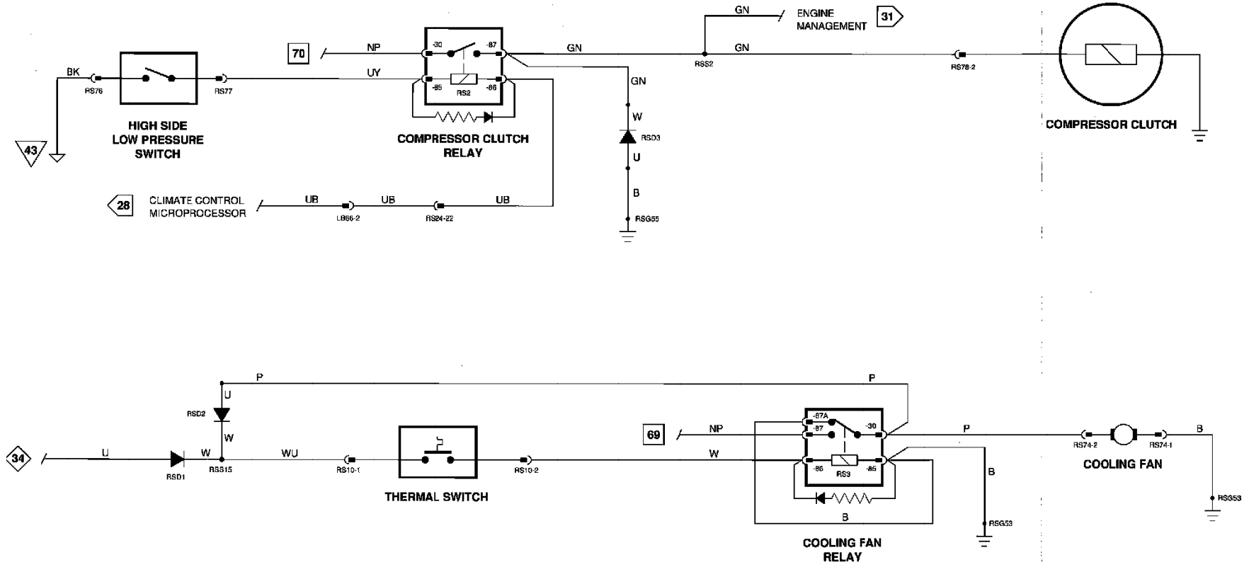
Compressor Clutch; Cooling Fan
