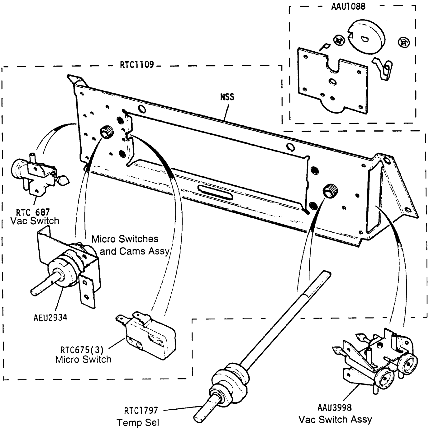
Complete heater assembly CAC2991
