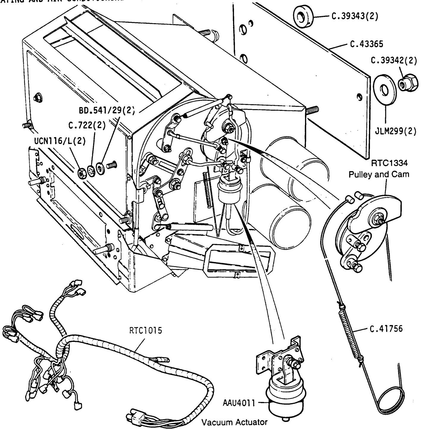
Complete heater assembly CAC2991
