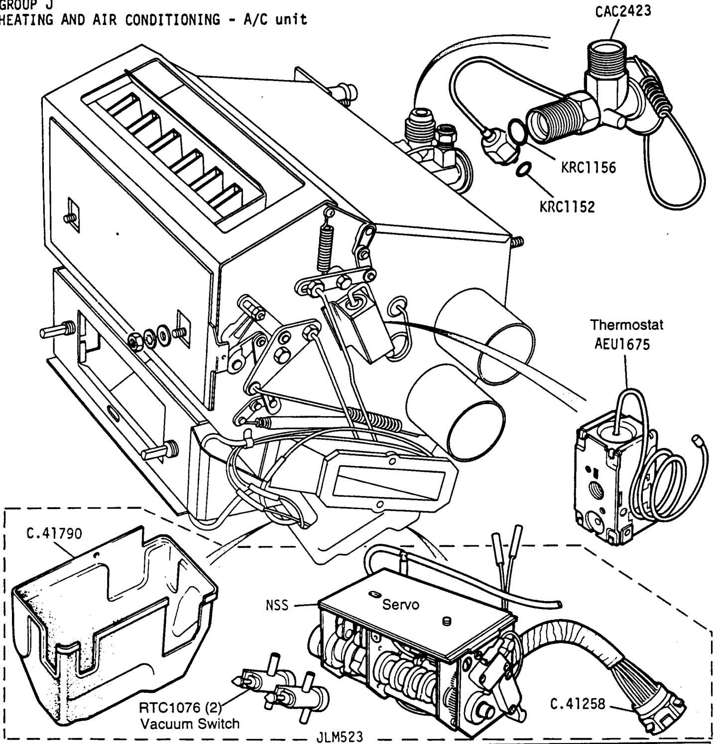
Complete A/C unit assembly CAC3660
