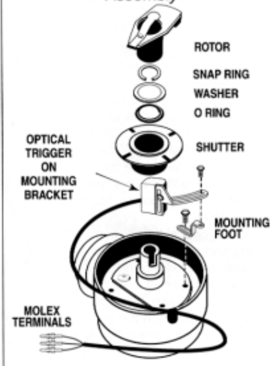
Figure 14. Typical Lucas Distributor Assembly
