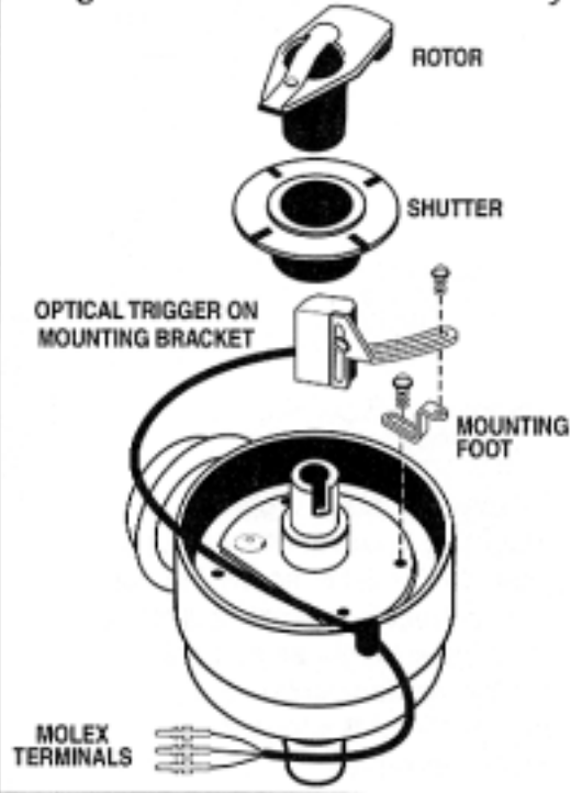
Figure 9. Distributor Assembly
