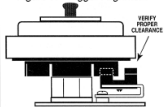
Figure 7. Trigger Alignment
