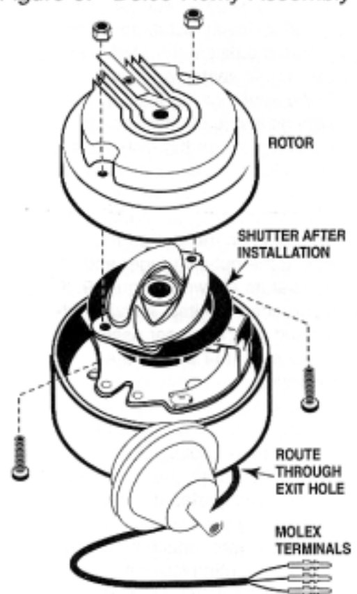
Figure 6. Delco-Remy Assembly
