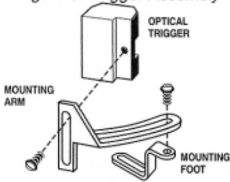
Figure 8. Trigger Assembly
