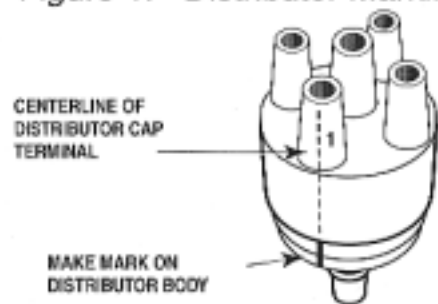
Figure 1. Distributor Marking
