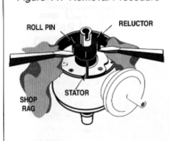
Figure 11. Removal Procedure
