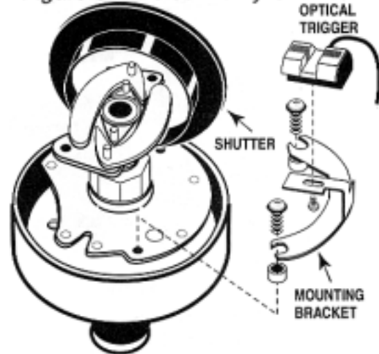
Figure 5. Delco-Remy Shutter
