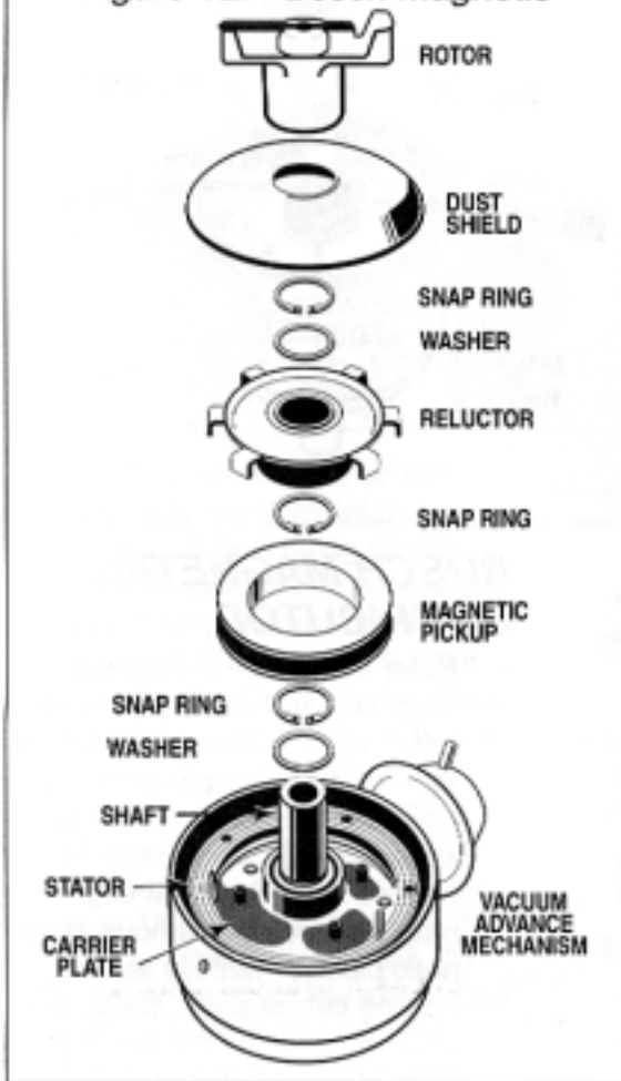
Figure 12. Bosch Magnetic
