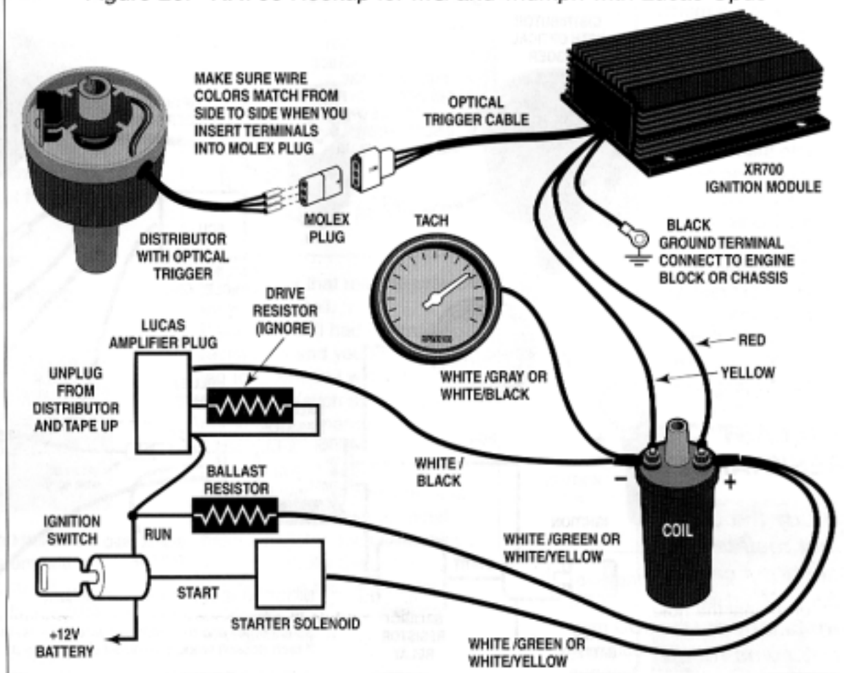
Figure 20. XR700 Hookup for MG and Triumph with Lucas Opus
