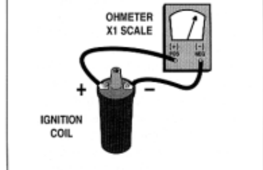
Figure 24. Coil Resistance Test
