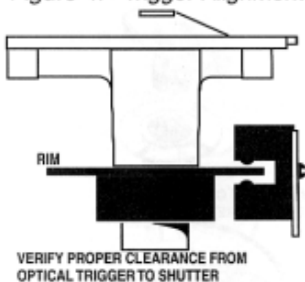
Figure 4. Trigger Alignment
