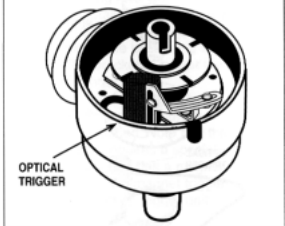
Figure 13. Hitachi Distributor
